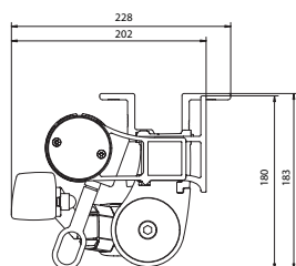
FA22 takmontering.
