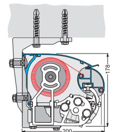
Family Basic takmontering (mm).
